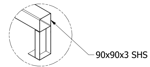
DETAIL C SCALE 1 : 12
