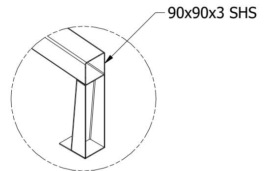
DETAIL C SCALE 1 : 12
