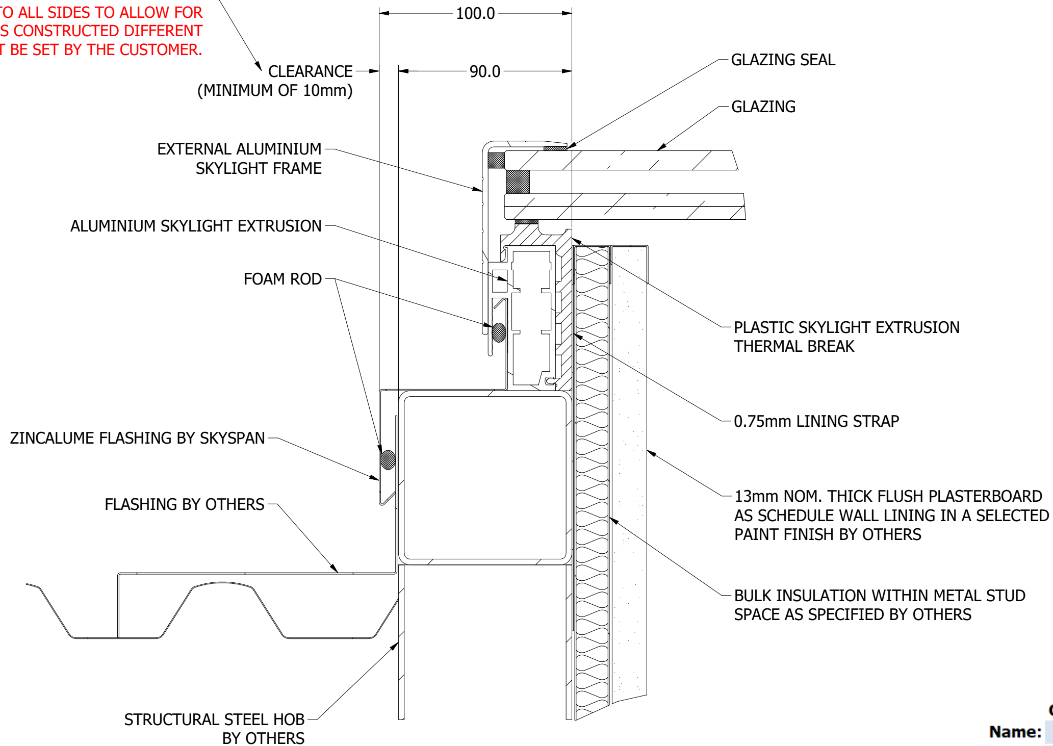
SECTION DETAIL VIEW SCALE 1 : 2
