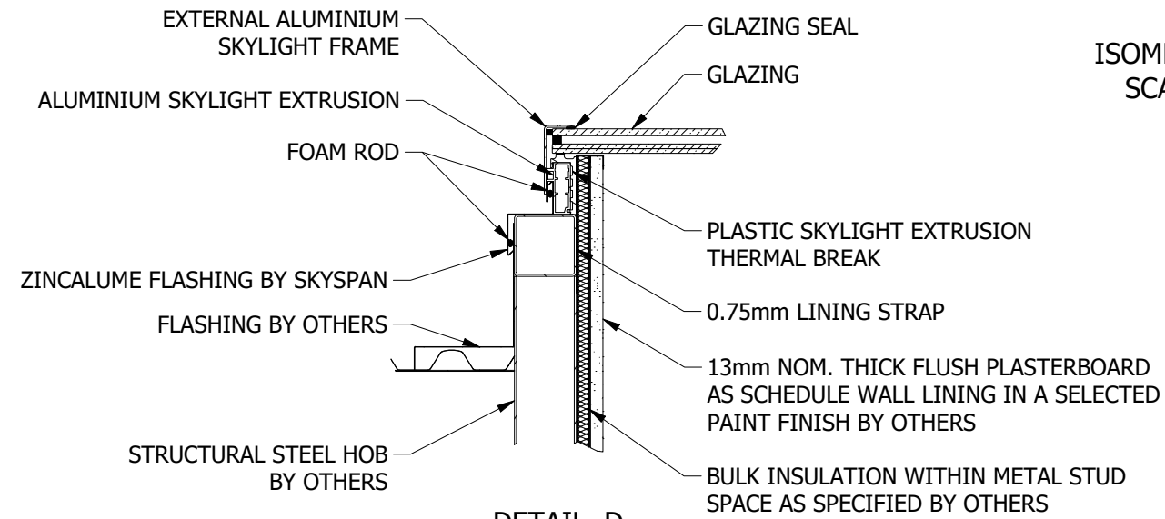
DETAIL D SCALE 1 : 10
