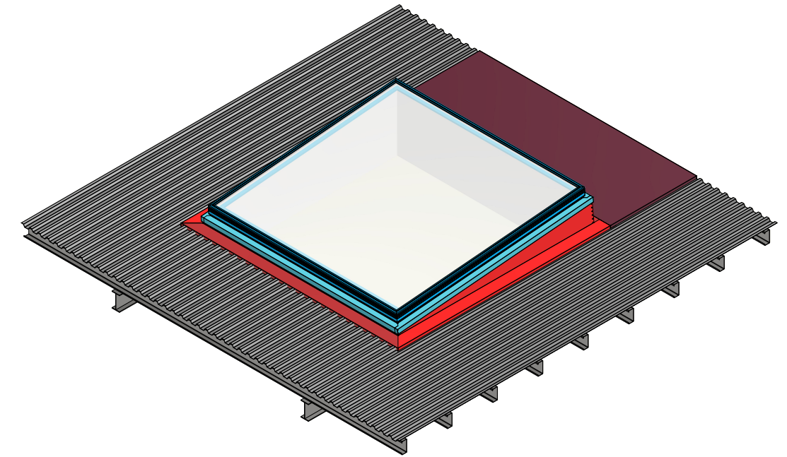
ISOMETRIC VIEW SCALE 1 : 50
